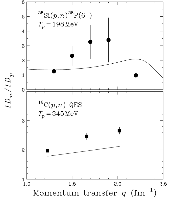
Fig. 4. Ratios of ID_n/ID_p for ^{28}\text{Si}(\vec{p}, \vec{n})^{28}\text{P}(6^-) at T_p = 198 MeV (upper panel) and quasielastic ^{12}\text{C}(\vec{p}, \vec{n}) at T_p = 345 MeV (lower panel). The solid curves are DWIA calculations with the free NN interaction, as described in the text.
