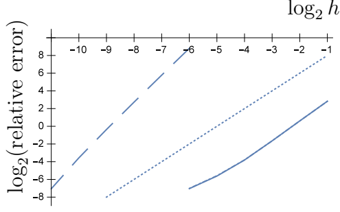
Figure 4: Log-log plot of the relative error of the variance versus h (Solid: SERKW2D2, dash-dotted: SERKW2D3, dash: SROCK2, dotted: reference line with slope 2)
