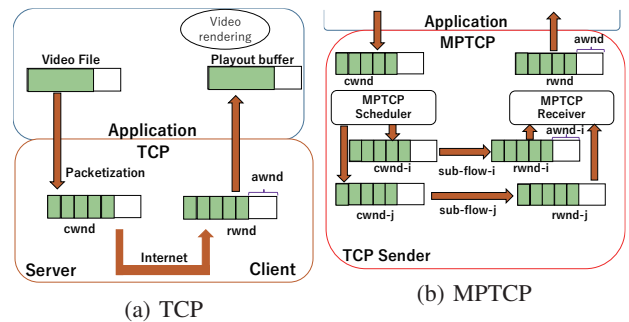
Figure 1: Video Streaming over TCP/MPTCP
