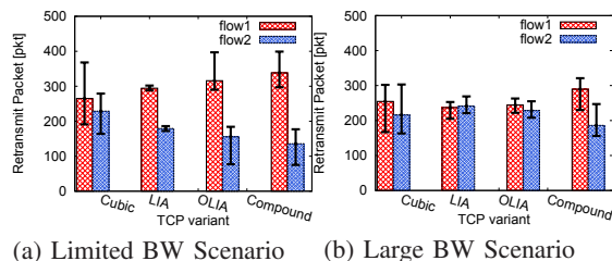
Figure 8: WiFi Handoff: transport retransmissions with GR-STY
