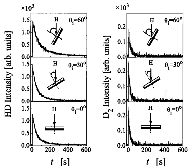
FIG. 2. Angle-integrated desorption rates of HD (left panel) and D 2 (right panel) molecules on the D/Si(100) surface at 473 K.
