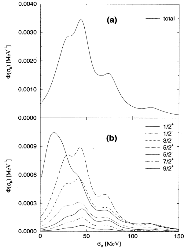
FIG. 1. The Lorentz transform of the longitudinal response function of {}^3\text{He} at |\vec{Q}| = 300 MeV/ c ( \sigma_I = 10 MeV); (a) the total sum of all channels contributions; (b) single channel contributions.
