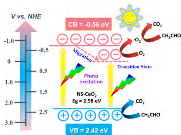
Fig. 7 A feasible mechanism for CH 3 CHO degradation by NS-CeO 2 photocatalyst.
