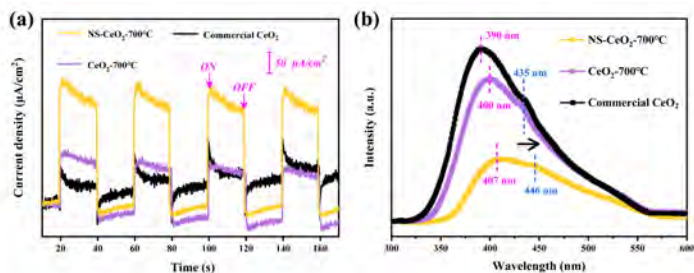
Fig. 4 (a) Transient photocurrent response and (b) steady-state photoluminescence spectra of NS-CeO 2 , pure CeO 2 and commercial CeO 2 .
