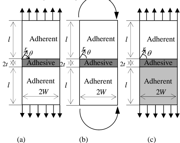
Fig.1 Adhesive joint under (a) tension, (b) bending (c) with different adherents under tension
