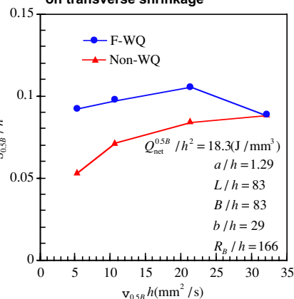
Fig.3 Effect of velocity parameter on transverse shrinkage
