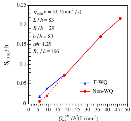
Fig.2 Effect of heat input parameter on transverse shrinkage
