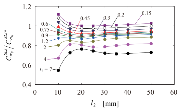
Figure 9. Relation between C_{\sigma_{ij}}^{SLJ} / C_{\sigma_{ij}}^{SLJ*} and l_2 .
