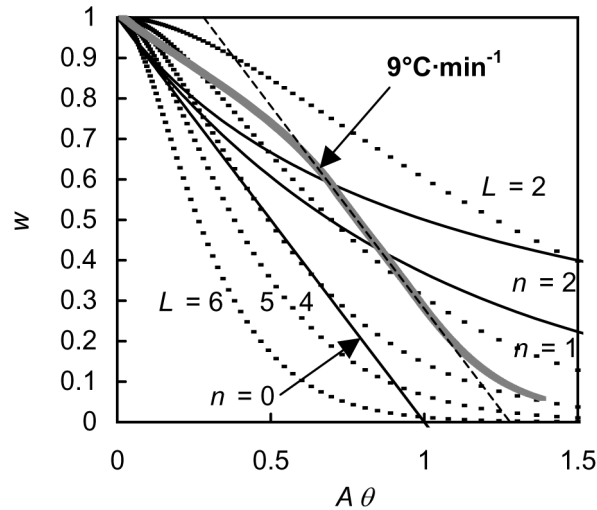
Figure 7. Plots of experimental A\theta vs. w for thermogravimetric data of PLLA/LLDPE/MgO [20:80:1 (wt/wt/wt)] in a range of w = 1.0-0.8 at a heating rate of 9\text{ }^{\circ}\text{C}\cdot\text{min}^{-1} and for model reactions using the kinetic parameters: E_a = 118\text{ kJ}\cdot\text{mol}^{-1} and A = 7.2\times 10^8\text{ s}^{-1} . Model reactions: zero ( n=0 ), 1 st ( n=1 ), and 2 nd ( n=2 )-order, and random degradations (Random L=2-6 ).
