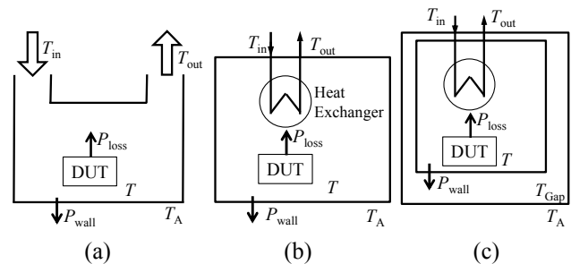
Fig. 1 Existing calorimetric measurement. (a) open type. (b) single-cased closed type. (c) double-cased closed type.
