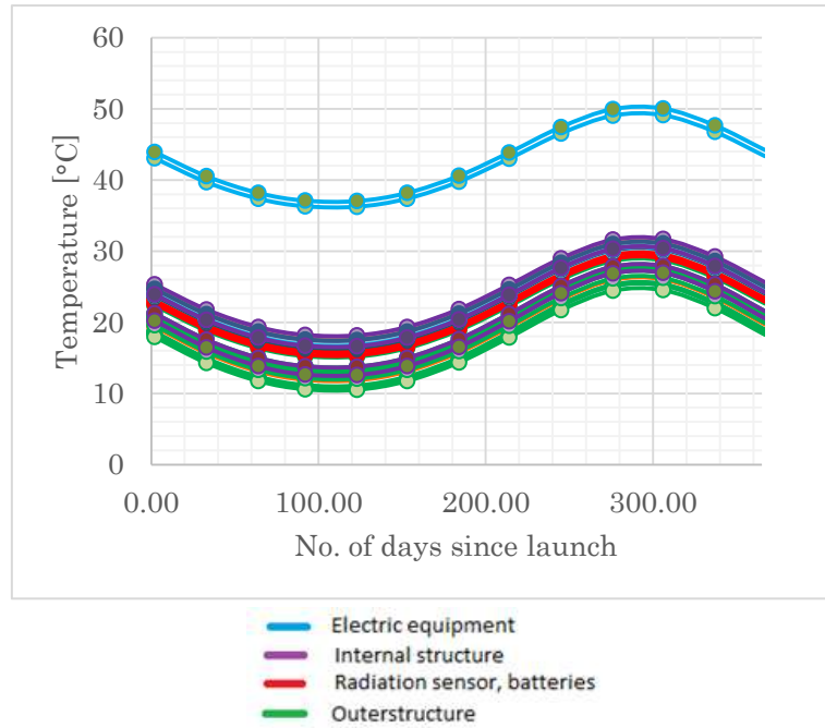
Figure 7 The analysis results in temperatures for one year period of time
