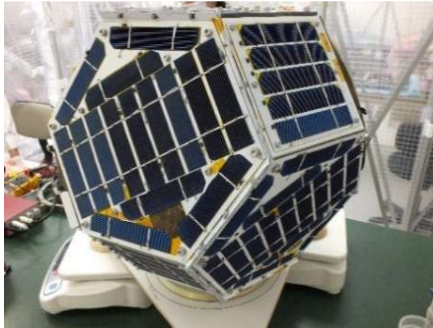
Figure 1 Flight model of Shinen2
