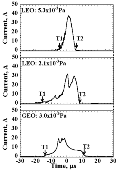
Fig. 5 Primary arc current waveforms of the Si cell in the LEO chamber and GEO chamber.
