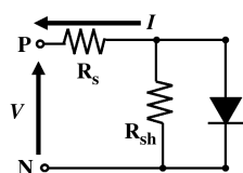
Fig. 13 Equivalent circuit of CIGS in dark condition.
