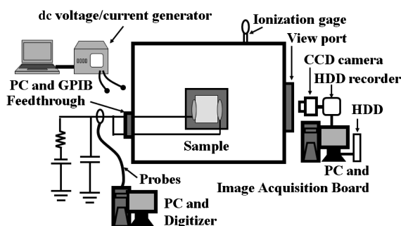
Fig. 3 Discharge experimental system, where HDD refers to the hard disk drive and GPIB refers to the general purpose interface bus.
