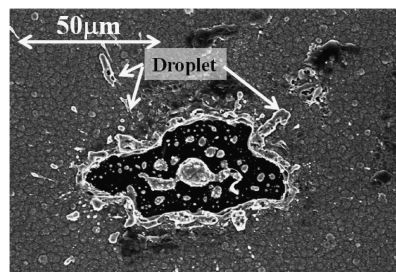
Fig. 25 Arc track not surrounded by an insulator.
