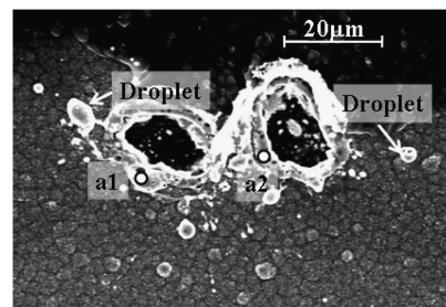
Fig. 22 SEM image of arc track on C06.
