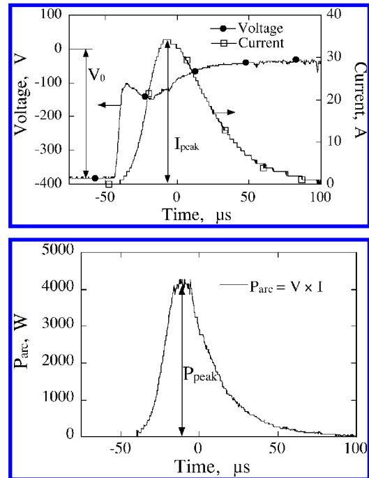
Fig. 13 Definitions of V_0 , I_{peak} , and P_{arc} .
