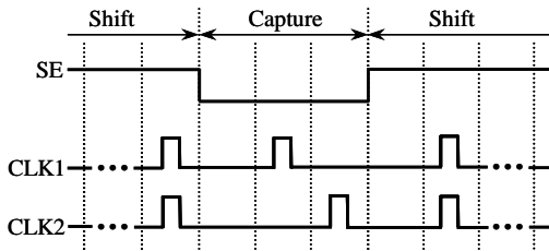
Fig. 4. Multi-Capture Clocking Scheme
