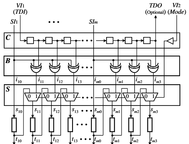
Fig. 3. Example Broadcaster
