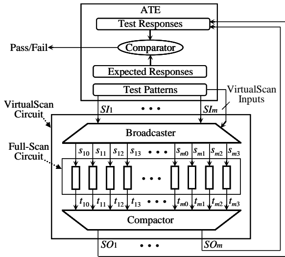
Fig. 1. VirtualScan Architecture
