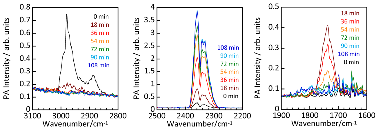
Figure 3. PA spectra of a TiO 2 film in an oxygen atmosphere containing 0.66 mmol L -1 of 2-propanol under UV irradiation.
