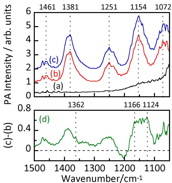
Figure 2. PA spectra of (a) TiO 2 powder in an oxygen atmosphere, (b) gaseous 2-propanol and (c) TiO 2 powder in an oxygen atmosphere containing 2-propanol, and (d) difference spectra of (c)-(b).
