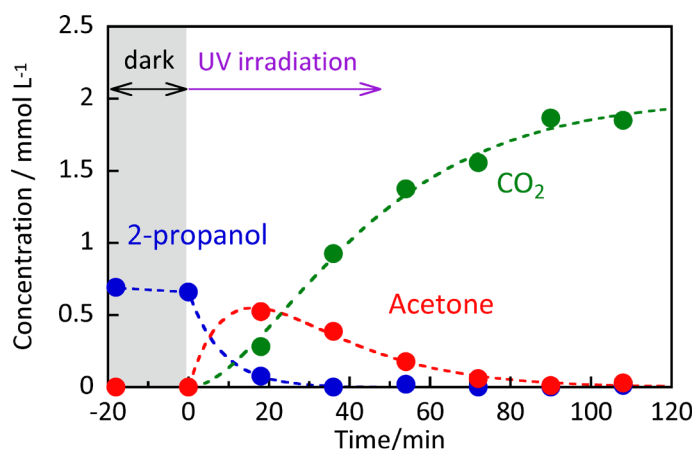
Figure 4. Time courses of concentrations of 2-propanol, acetone and CO 2 in the PA cell under photocatalytic reaction over a TiO 2 film.
