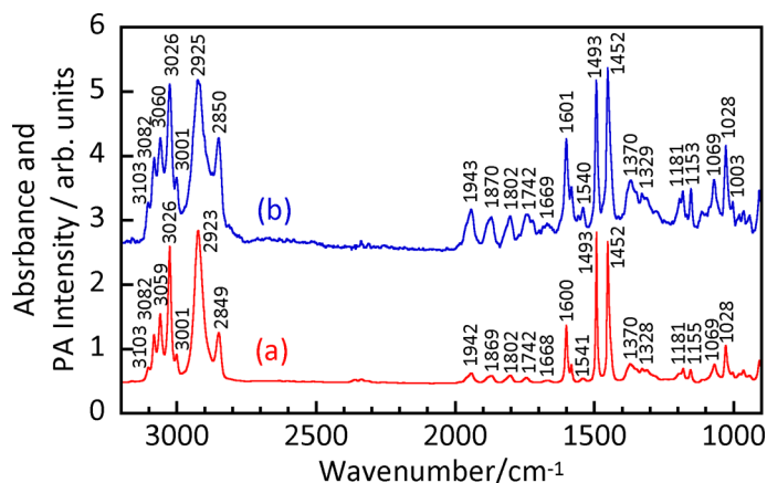
Figure 1. (a) FTIR spectra of polystyrene standard obtained by transmission and (b) PA spectrum of polystyrene foam.
