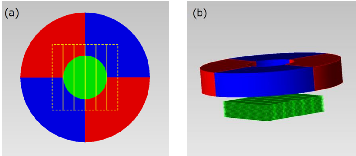
Figure 2. Calculation model for coated conductors as viewed from (a) above and (b) side.
