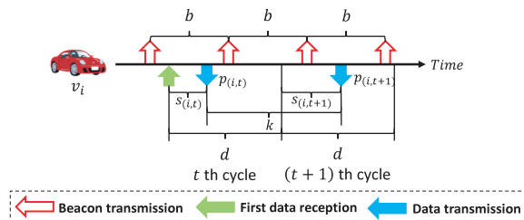
Fig. 2 Data transmission procedure
