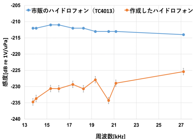
Fig.5 Frequency response of receiver sensitivity
